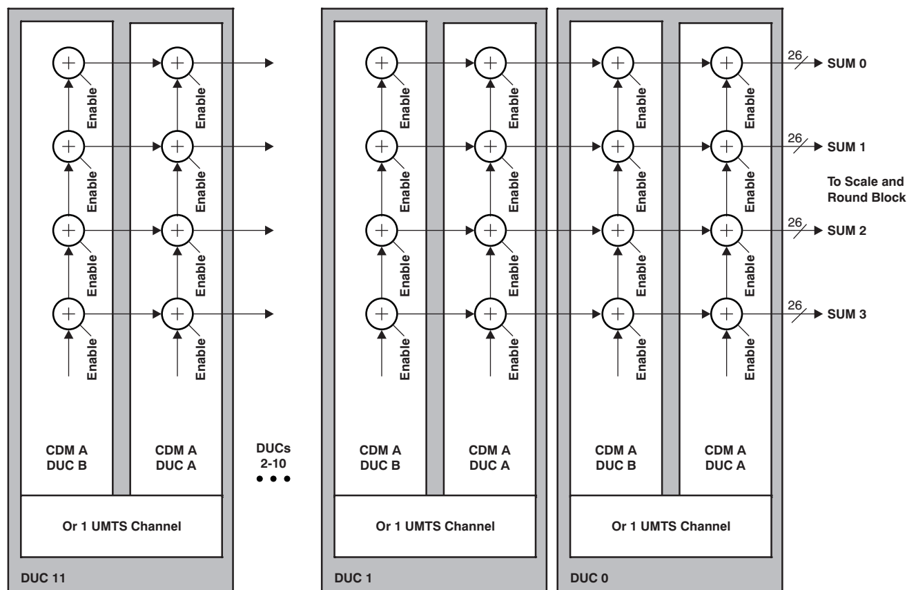
Figure 2-15. Sum Chain
